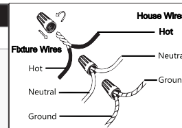
How to Identify the Fixture's Wires
